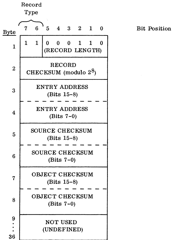
Figure 7-4. End Record Format
