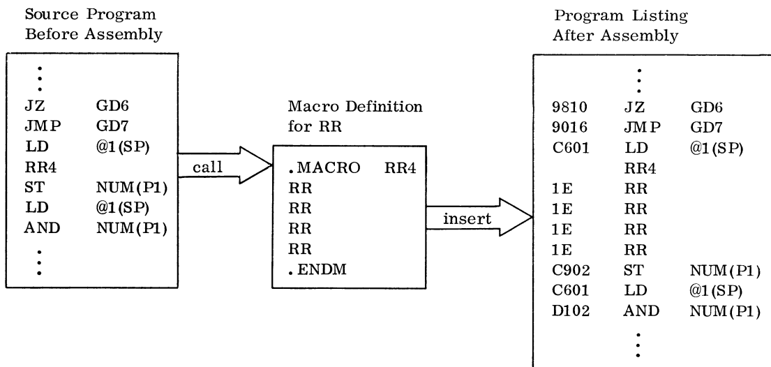
Figure 6-1. Statement Insertion
