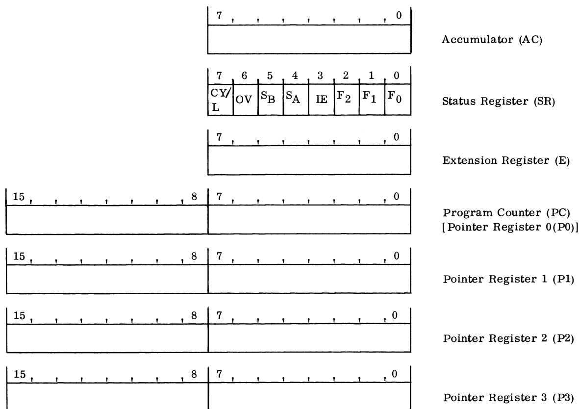
Figure 2-1. SC/MP Registers
