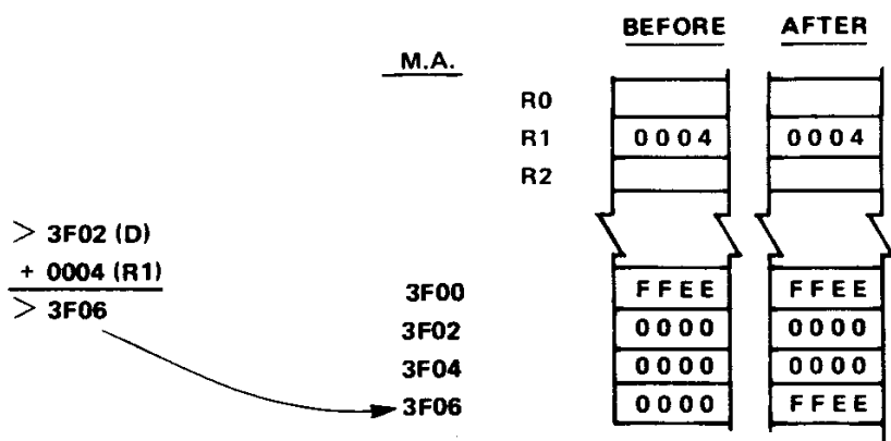
FIGURE 5-10. SYMBOLIC MEMORY ADDRESSING, INDEXED EXAMPLE
