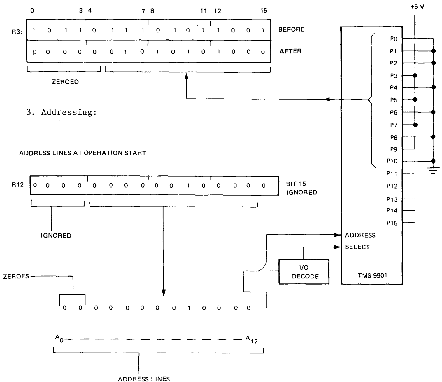
FIGURE 7-16. STCR WORD EXECUTION TO TMS 9901
