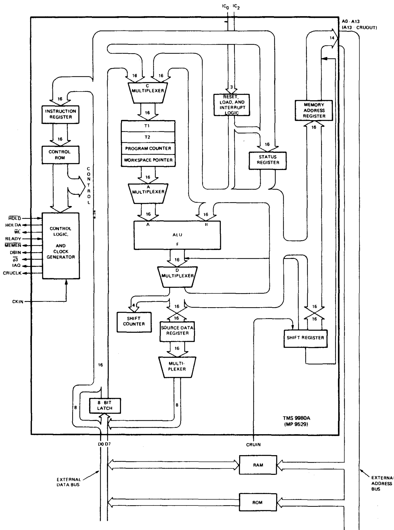
FIGURE 5-2. TMS 9980A WITH RAM/ROM MEMORY
