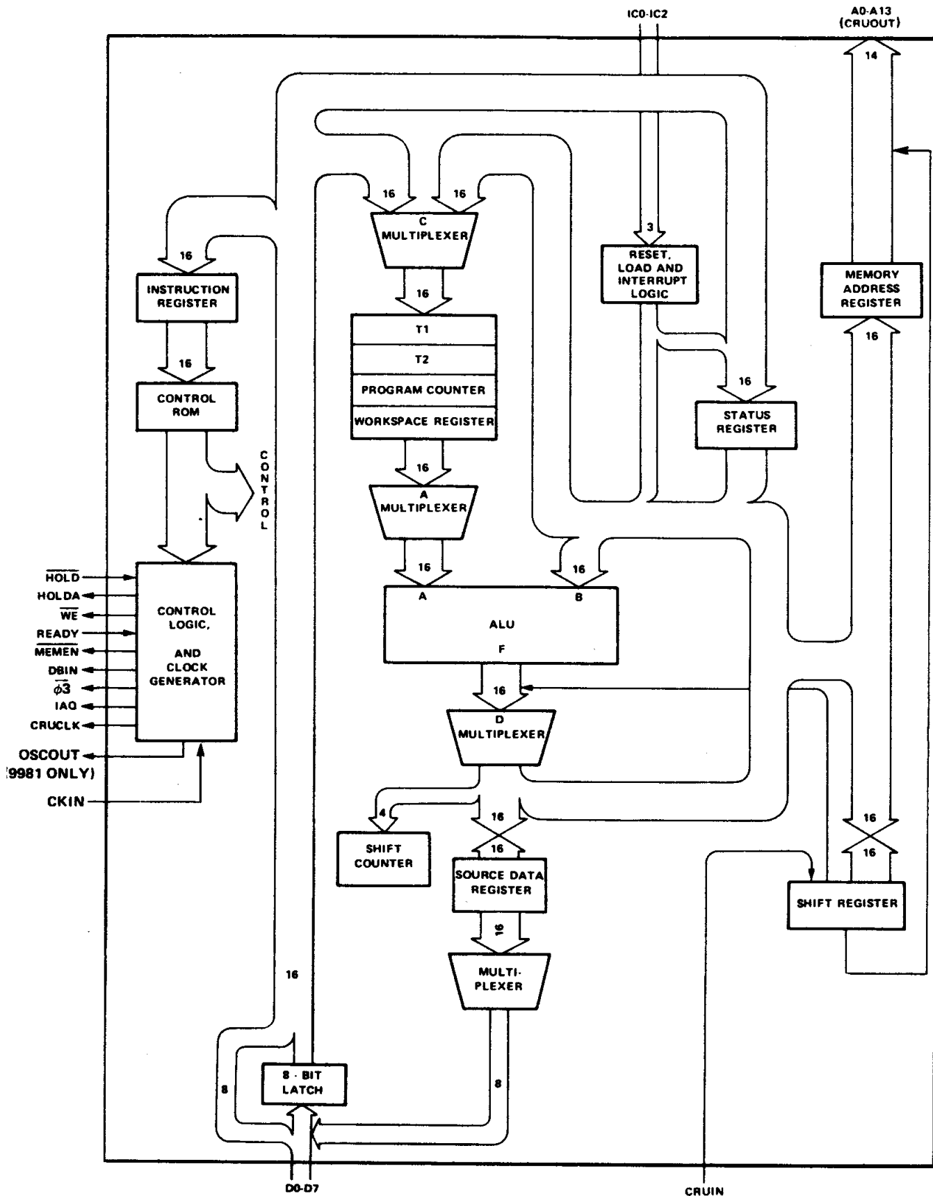
FIGURE 1 - ARCHITECTURE
