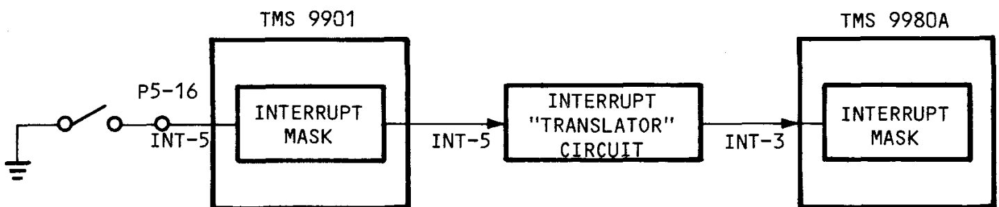
FIGURE 7-21. INTERRUPT PATH
