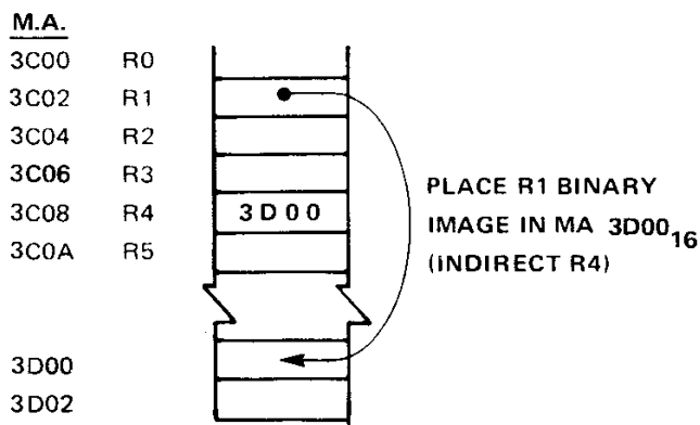
FIGURE 5-7. INDIRECT REGISTER ADDRESSING EXAMPLE
