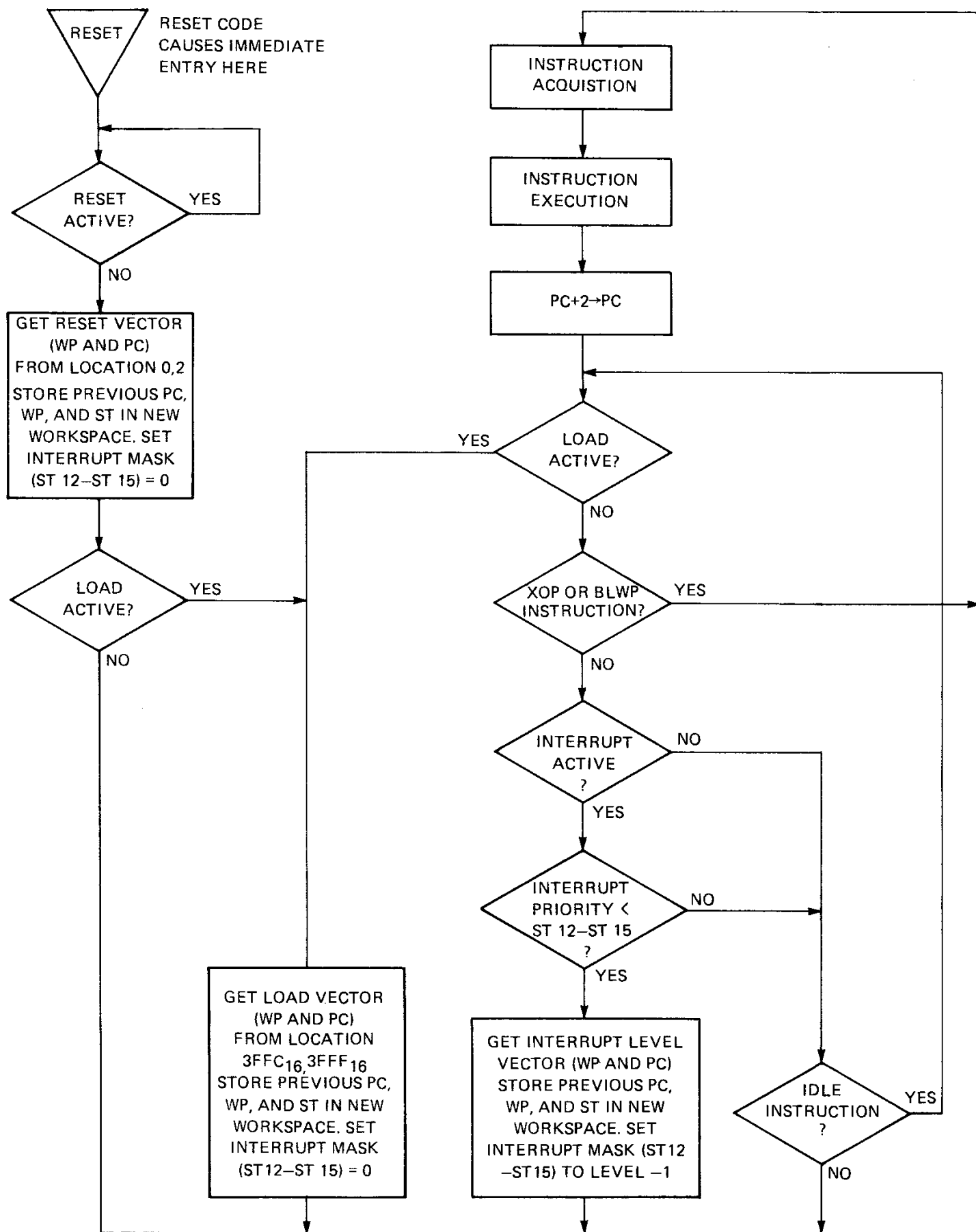
FIGURE 8-3. TMS 9980A CPU FLOW CHART
