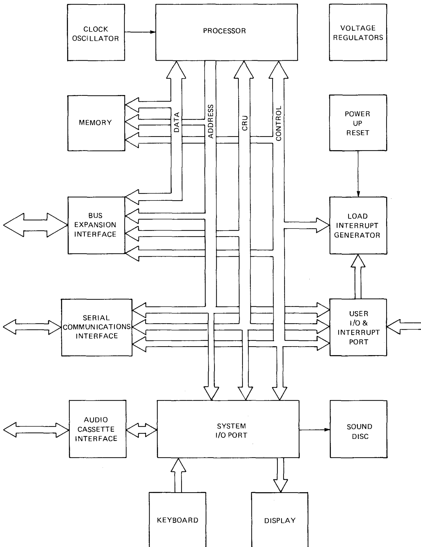
FIGURE 1-2. SYSTEM BLOCK DIAGRAM
