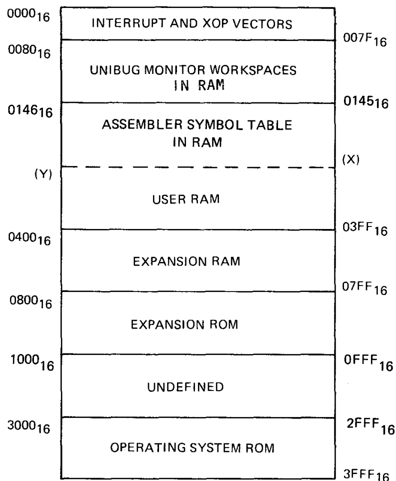
FIGURE 5-1. MEMORY MAP
