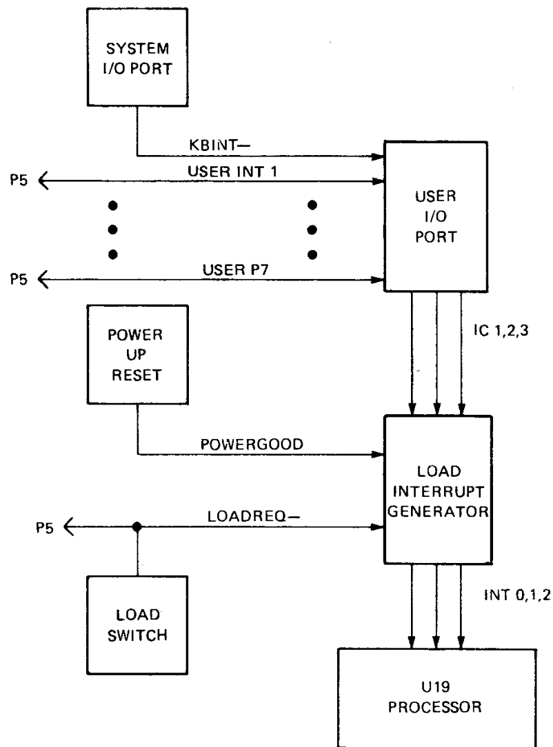
FIGURE 8-6. INTERRUPT SIGNAL FLOW
