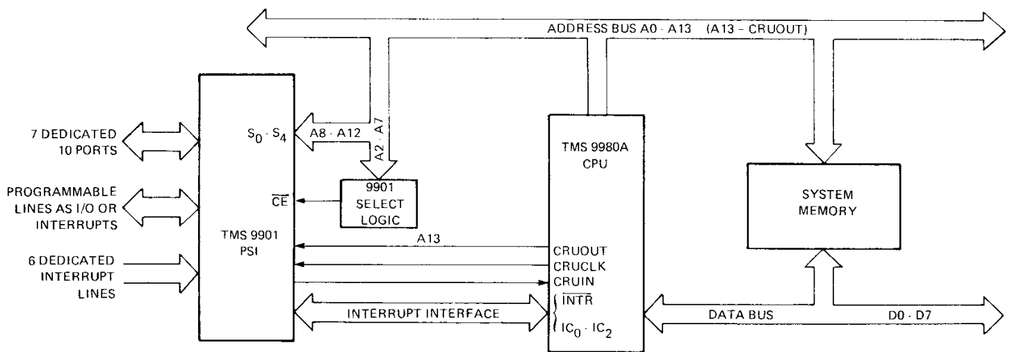
FIGURE 7-2. TYPICAL TMS 9901 PROGRAMMABLE SYSTEM INTERFACE (PSI) APPLICATION
