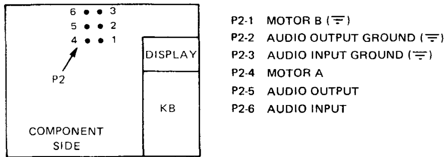
FIGURE 2-9. ACI CONNECTOR PINS
