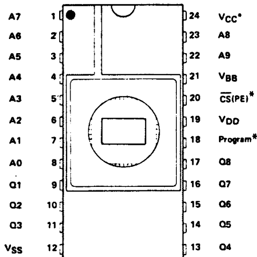
24-PIN CERAMIC DUAL-IN-LINE PACKAGE (TOP VIEW)
