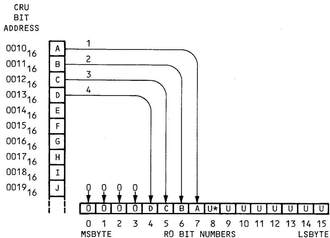
FIGURE 7-9. STCR WORD TRANSFER
