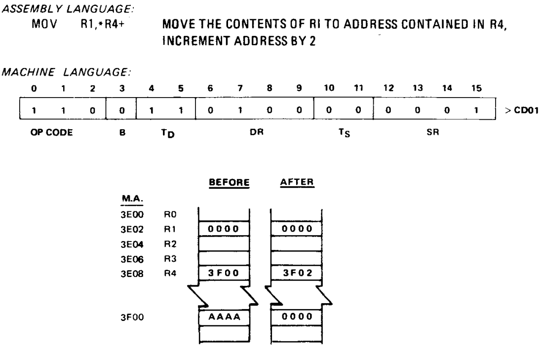
FIGURE 5-8. INDIRECT REGISTER AUTOINCREMENT ADDRESSING EXAMPLE
