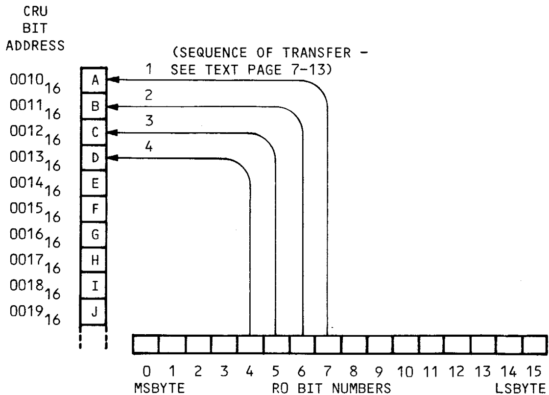
FIGURE 7-8. LDCR BYTE TRANSFER
