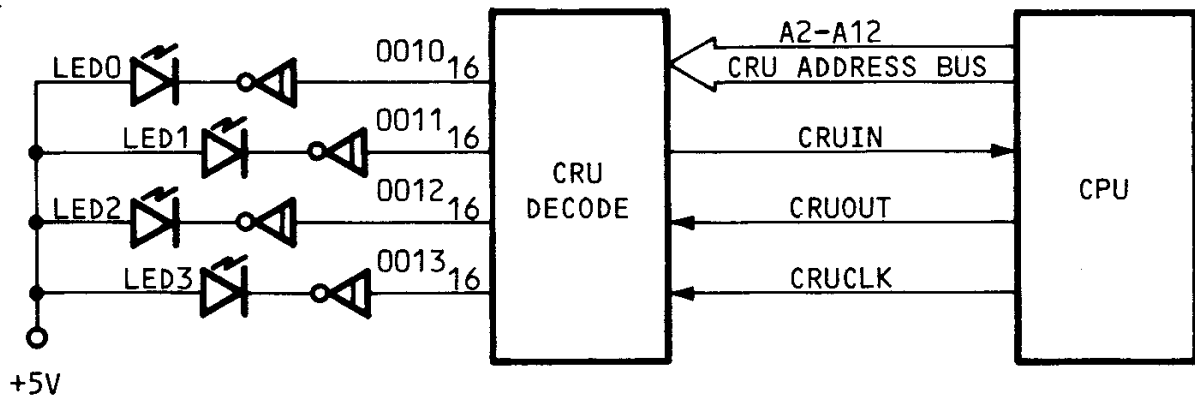
FIGURE 7-5. ADDRESSING ONBOARD LEDS
