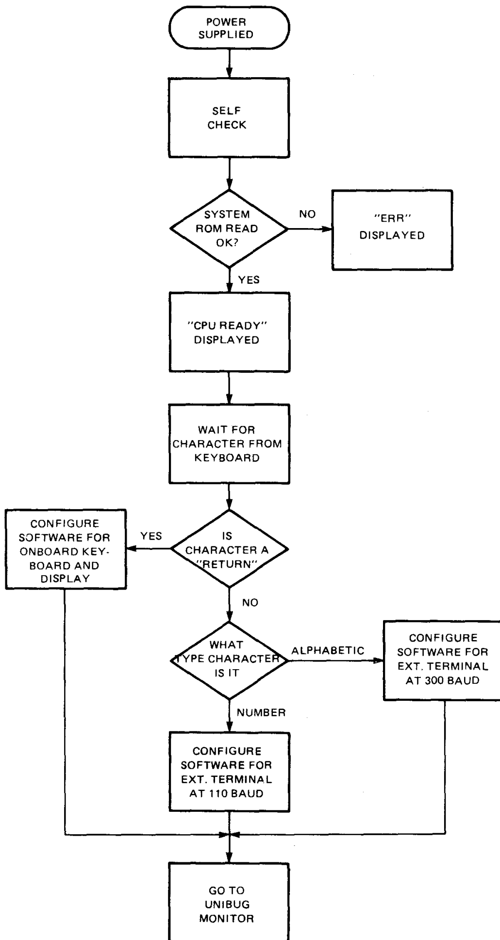
FIGURE 2-4. POWER UP INITIALIZATION FLOW CHART
