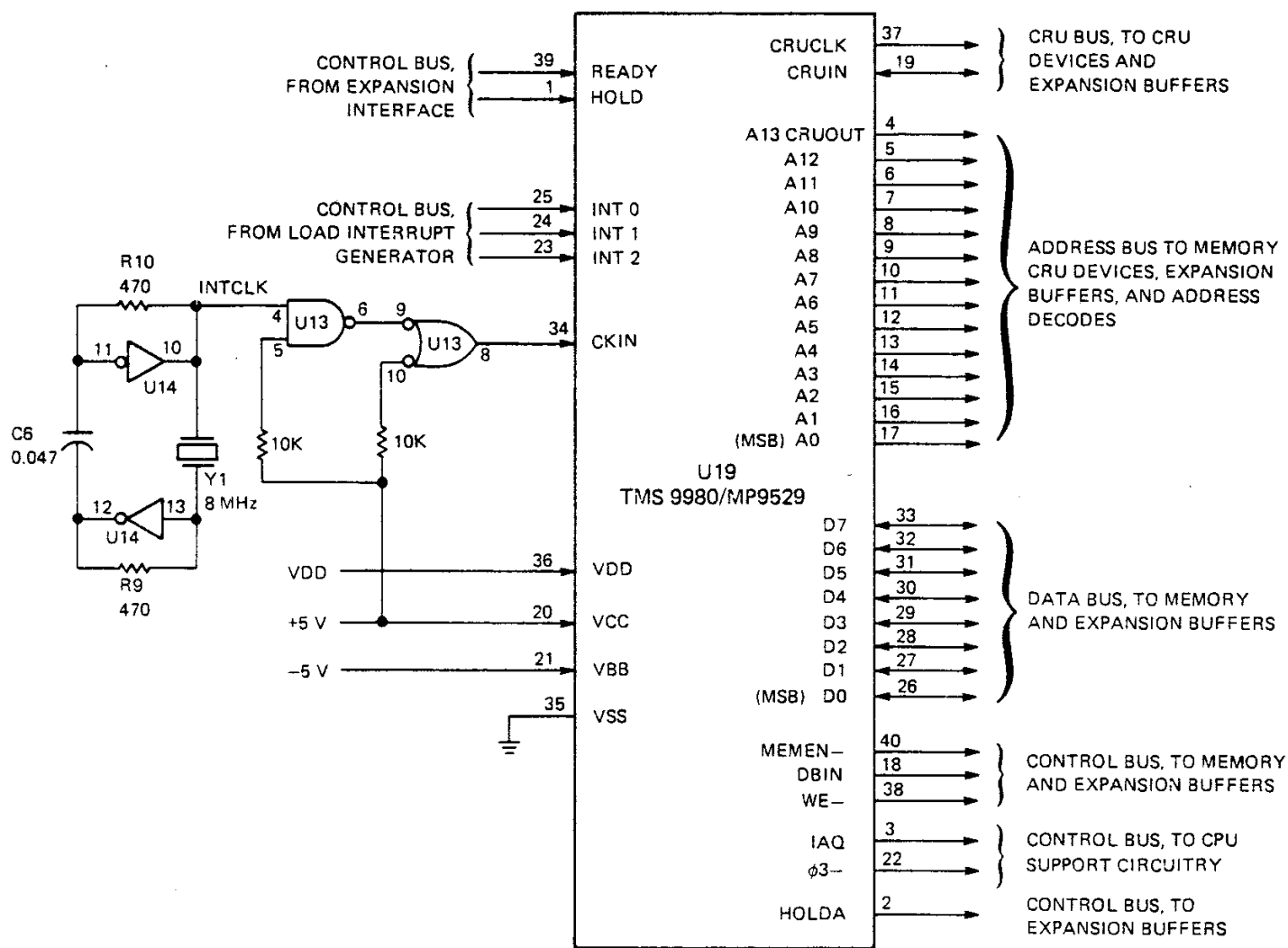
FIGURE 8-4. TMS 9980A SIGNALS
