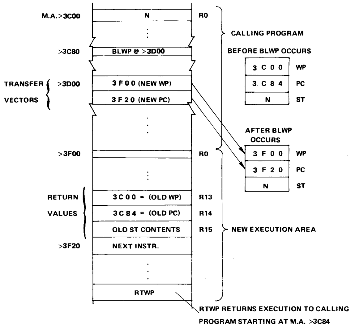
FIGURE 5-11. BLWP EXAMPLE
