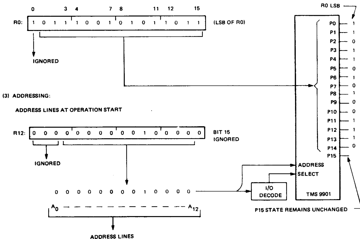
FIGURE 7-14. LDCR WORD EXECUTION TO TMS 9901
