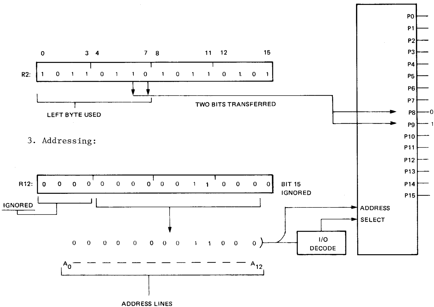
FIGURE 7-15. LDCR BYTE EXECUTION TO TMS 9901
