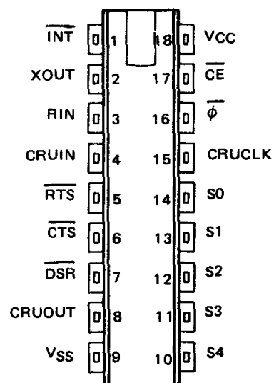
TMS 9902 18-PIN PACKAGE
