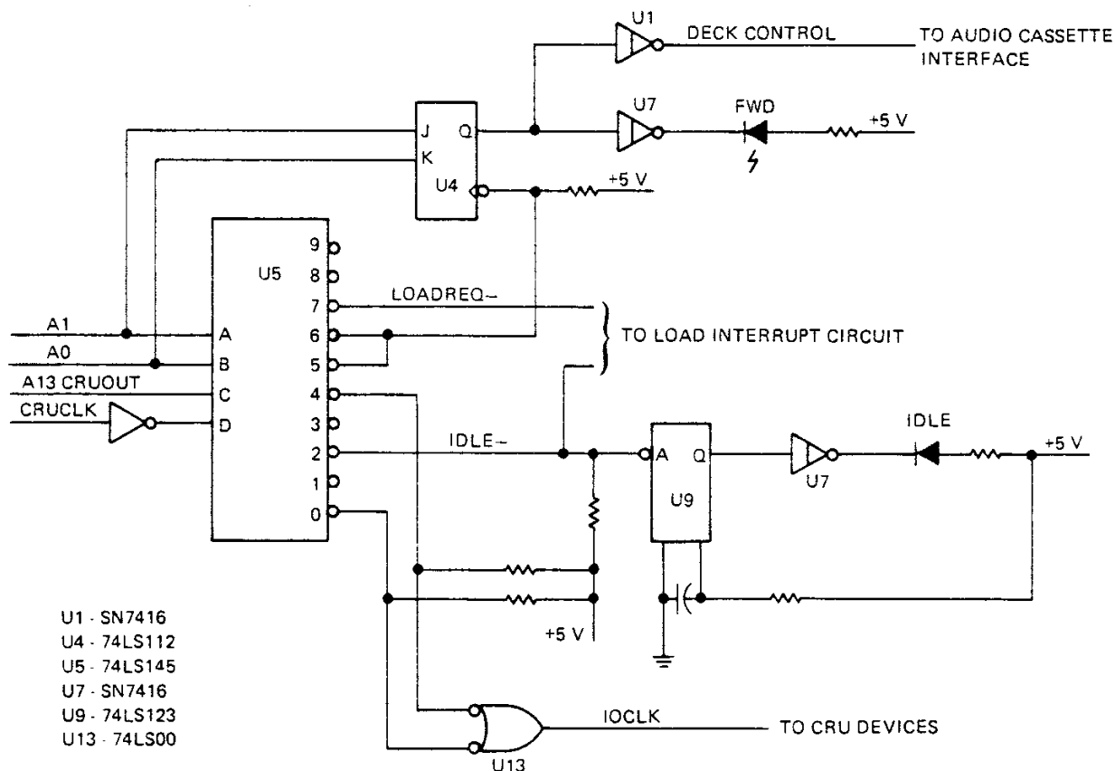
FIGURE 8-5. EXTERNAL INSTRUCTION DECODE
