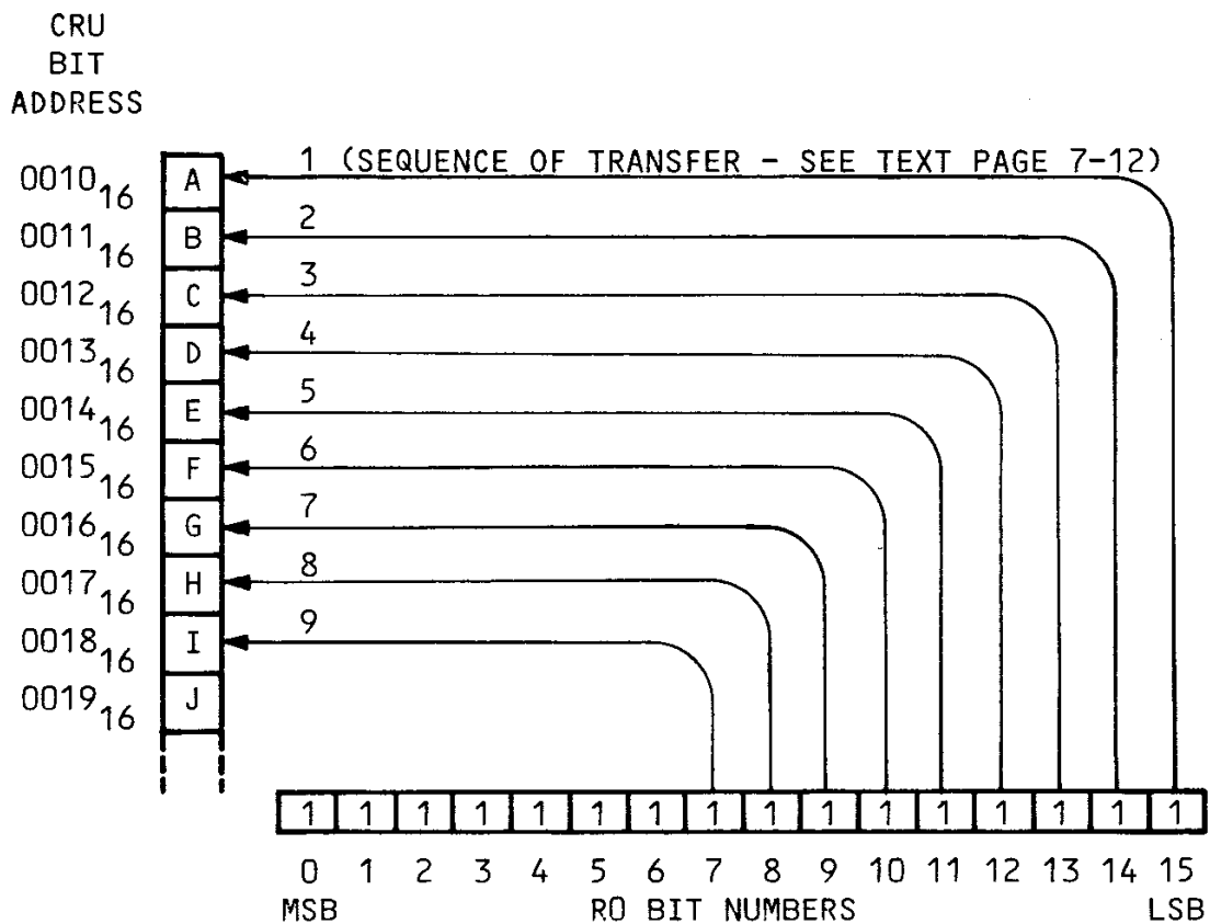
FIGURE 7-7. LDCR WORD TRANSFER
