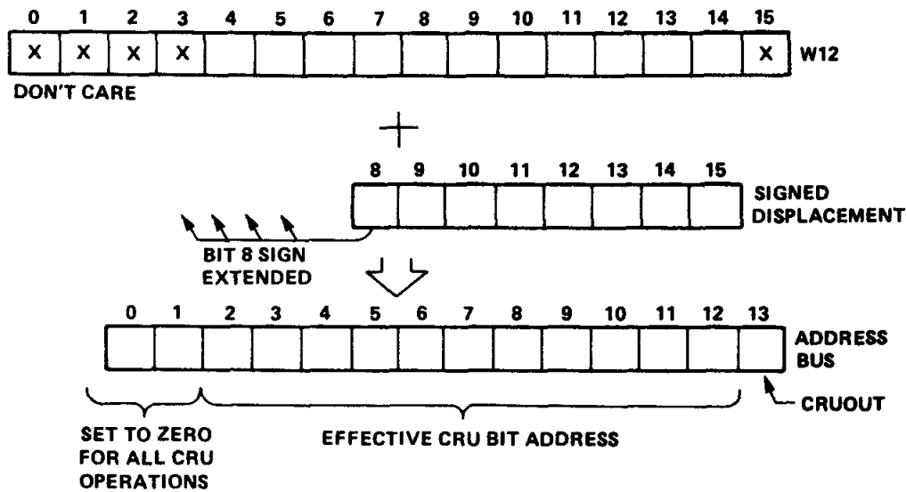
FIGURE 4 – TMS 9980A/TMS 9981 SINGLE-BIT CRU ADDRESS DEVELOPMENT
