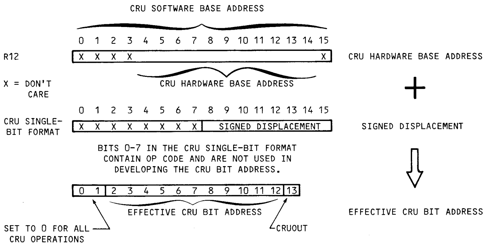
FIGURE 7-3. CRU BASE AND BIT ADDRESS
