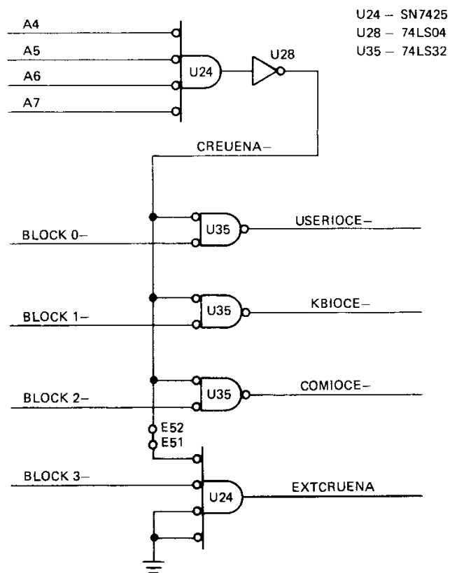
FIGURE 8-17. CRU ADDRESS DECODING LOGIC
