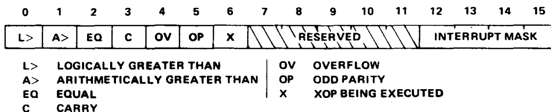
FIGURE 5-3. STATUS REGISTER
