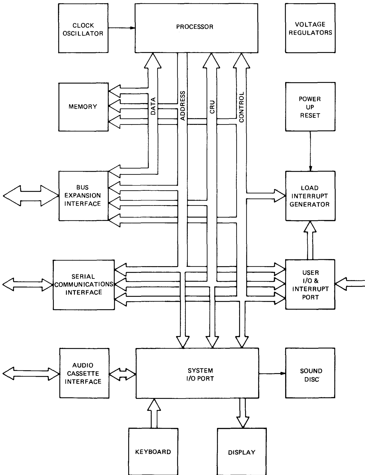
FIGURE 8-1. SYSTEM BLOCK DIAGRAM
