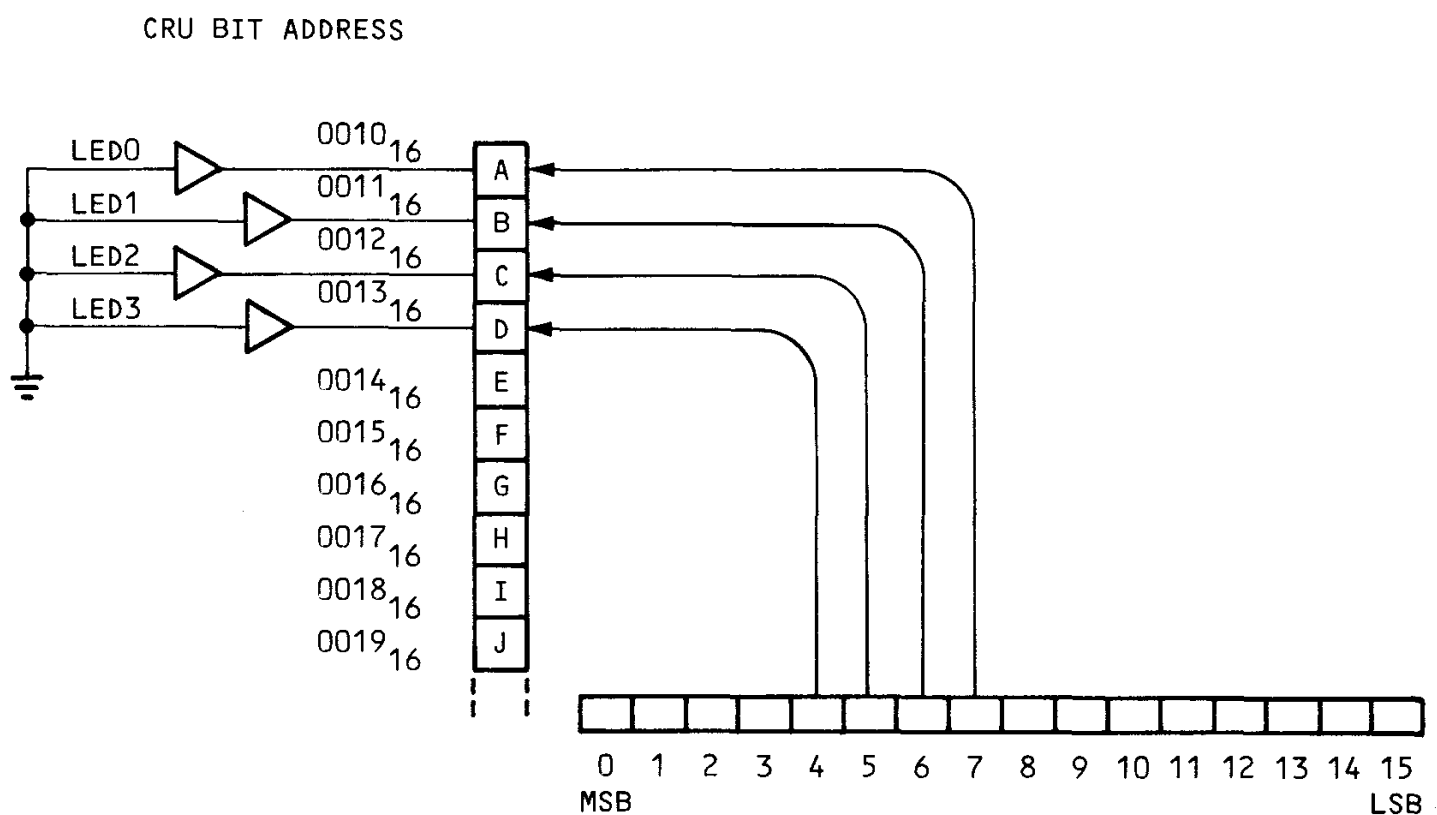
FIGURE 7-13. LDCR BYTE TRANSFER EXAMPLE
