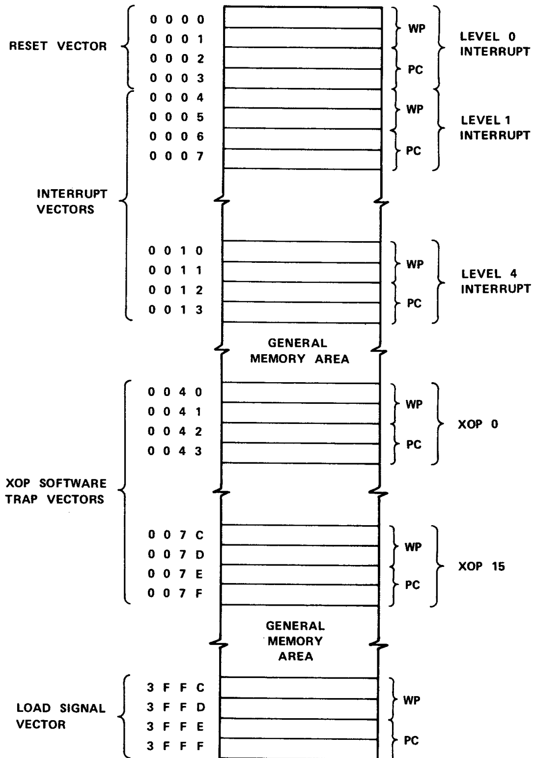
FIGURE 2 – MEMORY MAP
