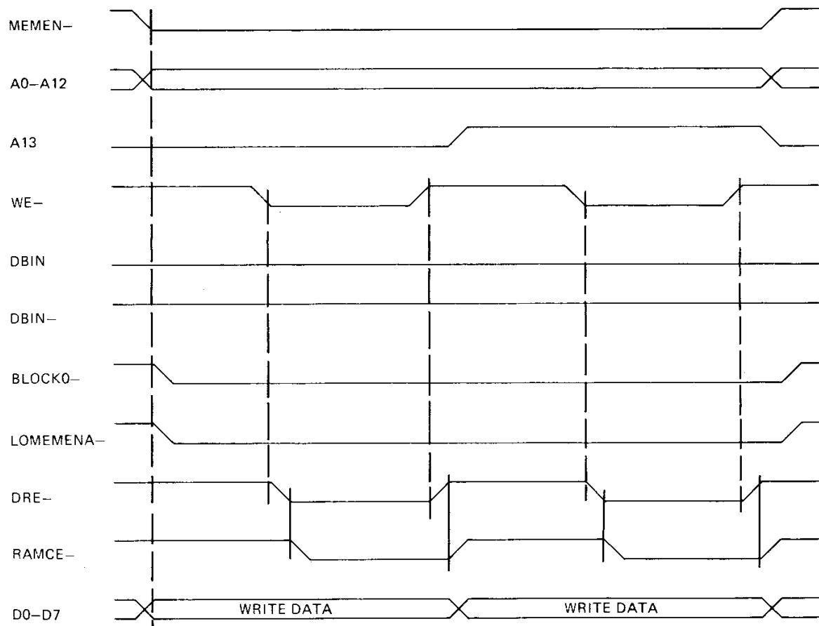
FIGURE 8-14. RAM WRITE CYCLE TIMING
