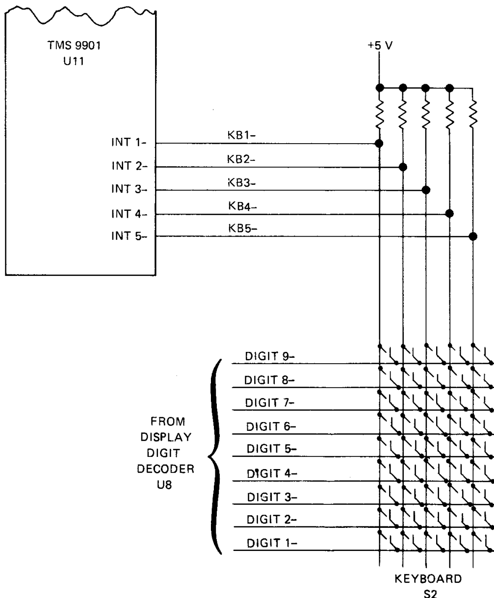
FIGURE 8-21. KEYBOARD INTERFACE
